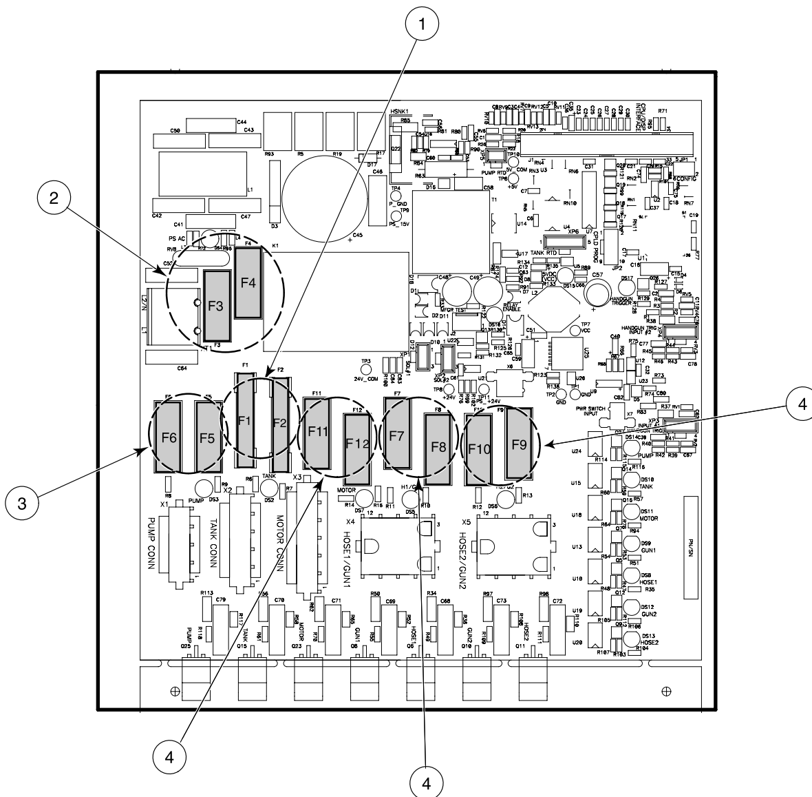
Figure 7-18 Fuse service kit parts
